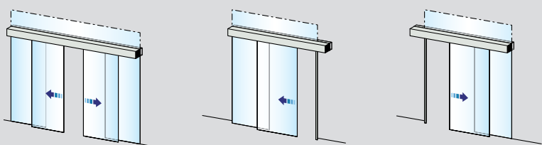
Beam mounted, doors and side screens (option overhead)
